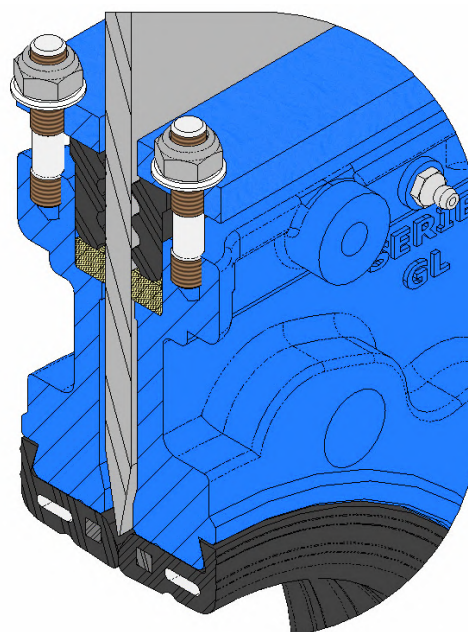
DETAIL-G
