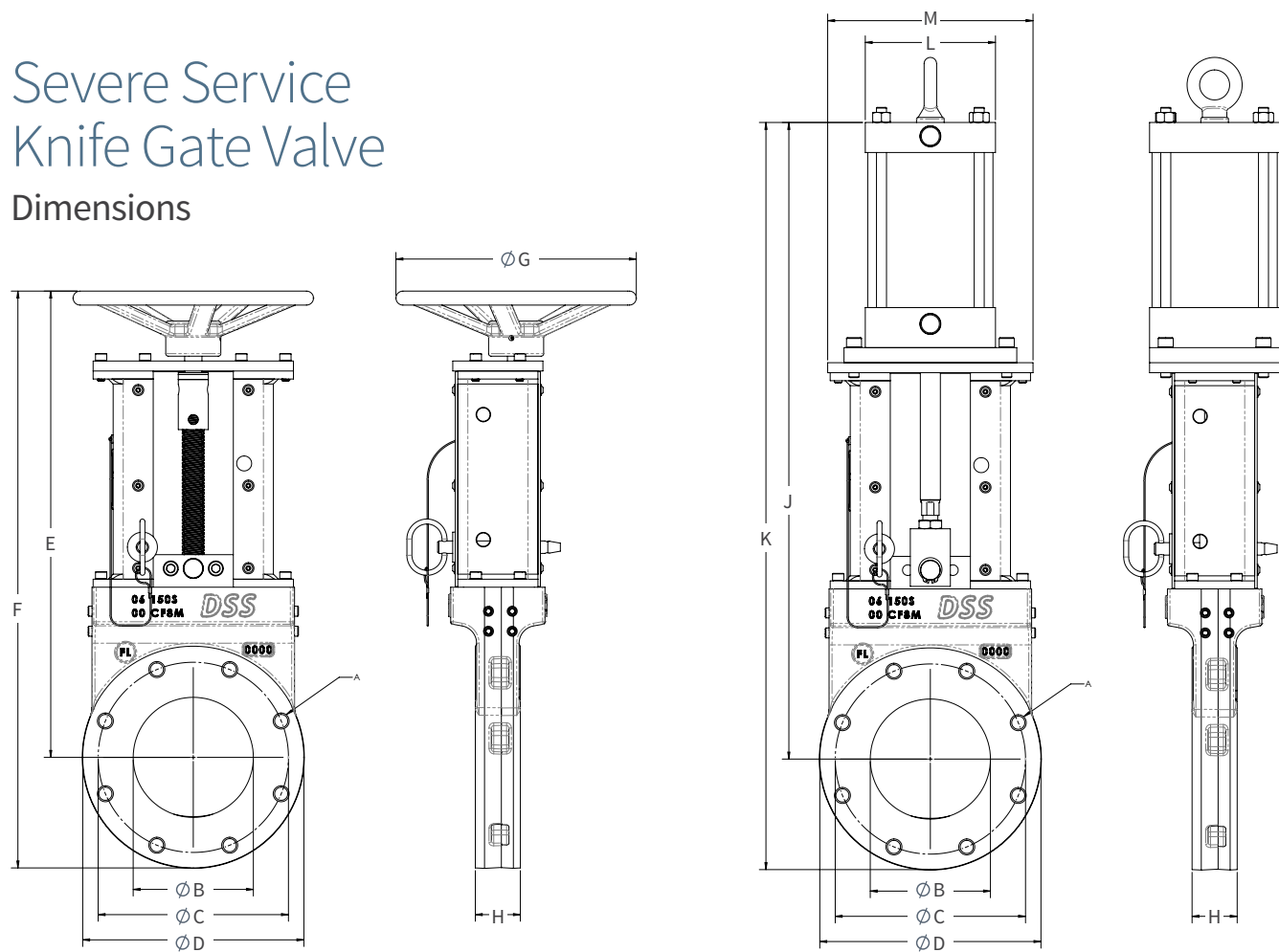
SSKGV CLASS 150 DIMENSIONS
