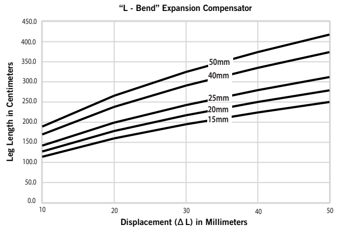
"L-Bend" Expansion Compensator Figure 1
